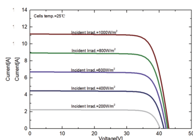
I-V Curves of SP-375Q at different irradiance
