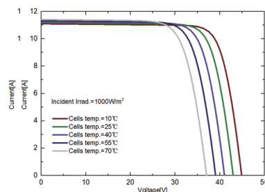
I-V Curves of SP-375Q at different cell temperature
